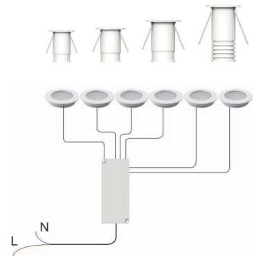
Connect to 110V or 230V
